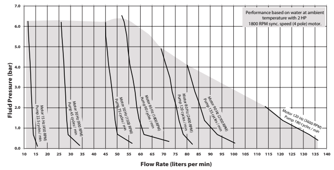
E2P10-XXXX-CX-XXA Maximum Outlet Working Pressure 190 PSIG (13.1 bar). End user piping design must be rated to withstand this pressure.
