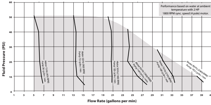
E2P10-XXXX-AX-XXA Maximum Outlet Working Pressure 100 PSIG (6.89 bar). End user piping design must be rated to withstand this pressure.
