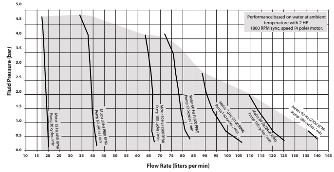
E2P10-XXXX-BX-XXA Maximum Outlet Working Pressure 140 PSIG (9.65 bar). End user piping design must be rated to withstand this pressure.
